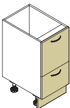
BD400R1D 400 Base Rubbish Bin Unit 870H x 400W x 588D Twin Bin Fitted
