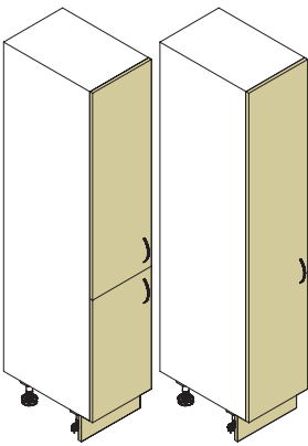
P400 400 Pantry Unit 2086H x 400W x 588D Options: P4002D – 2 Door P400PO – Pull Out Unit P400SPO – Swivelling Pull Out Unit
