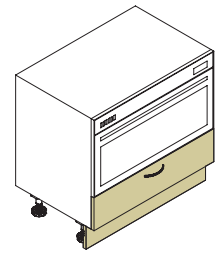
UBO9001DR 900 Underbench Oven Unit 870H x 900W x 588D
