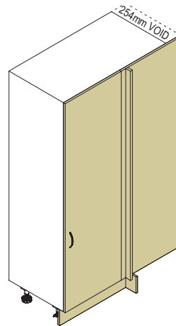
PR1000 1000 Pantry Return Unit 2086H x 1000W x 588D Options: PR1000BF – Bi-Fold Doors
