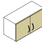
WOF700 700 Wall Over Fridge Unit 368H x 700W x 318D
